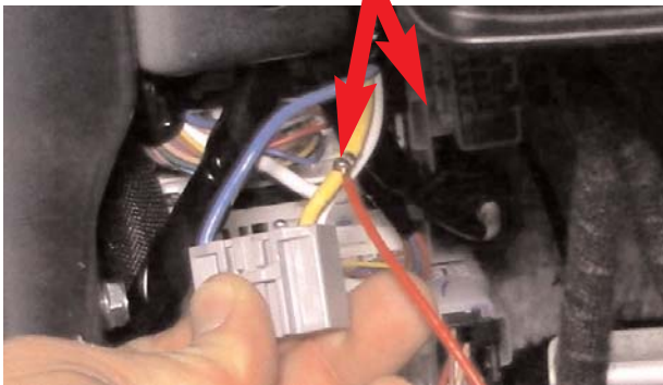
Below drivers dash near kick panel locate Gray connector in position 1 connect cruise red ignition wire to yellow wire for ignition power. Connector view shown unplugged with arrow pointing back to its location
